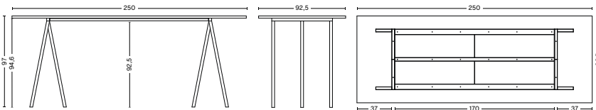
LOOP STAND TABLE HIGH WITH SUPPORT | L250 LENGTH 250 CM WIDTH 92,5 CM HEIGHT 97 CM TABLETOP THICKNESS 2,4 CM
