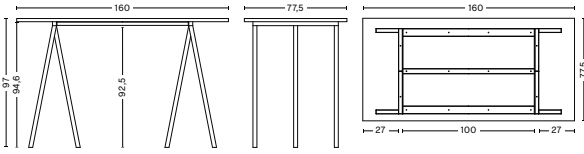
LOOP STAND TABLE HIGH WITH SUPPORT | L160 LENGTH 160 CM WIDTH 77,5 CM HEIGHT 97 CM TABLETOP THICKNESS 2,4 CM
