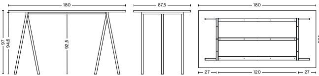
LOOP STAND TABLE HIGH WITH SUPPORT | L180 LENGTH 180 CM WIDTH 87,5 CM HEIGHT 97 CM TABLETOP THICKNESS 2,4 CM
